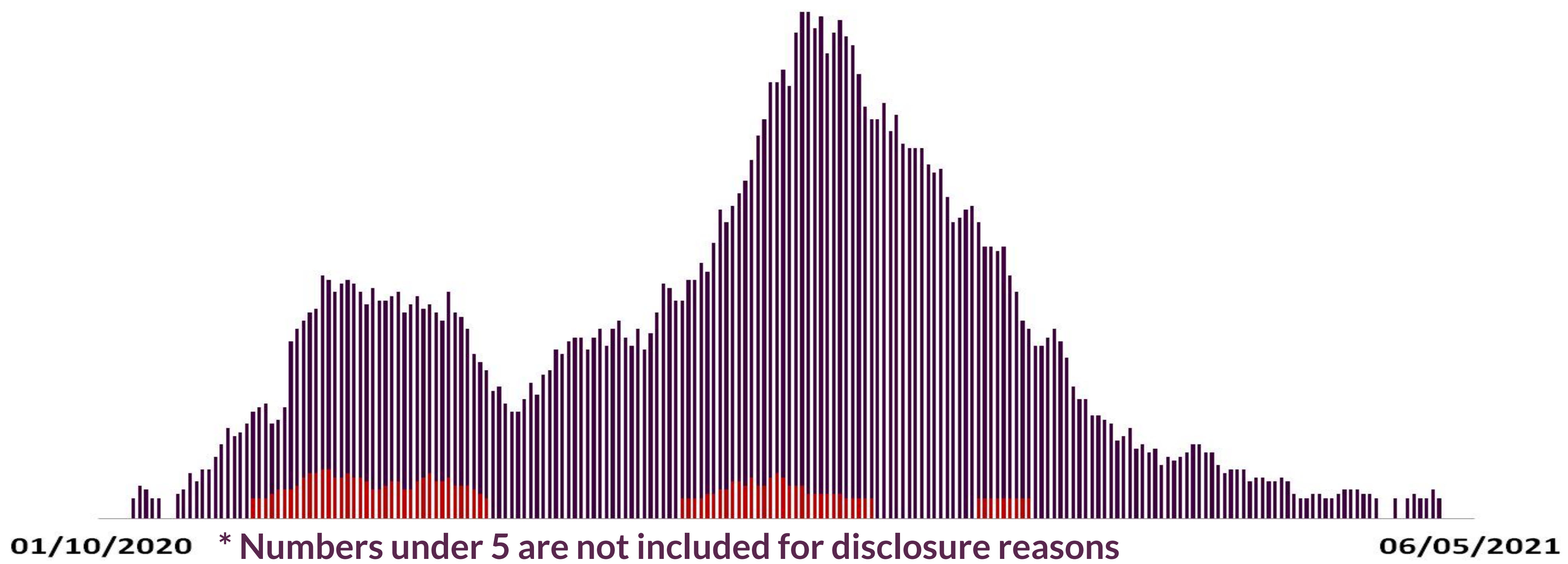
Daily number of people in hospital with recently confirmed COVID-19 in Fife
