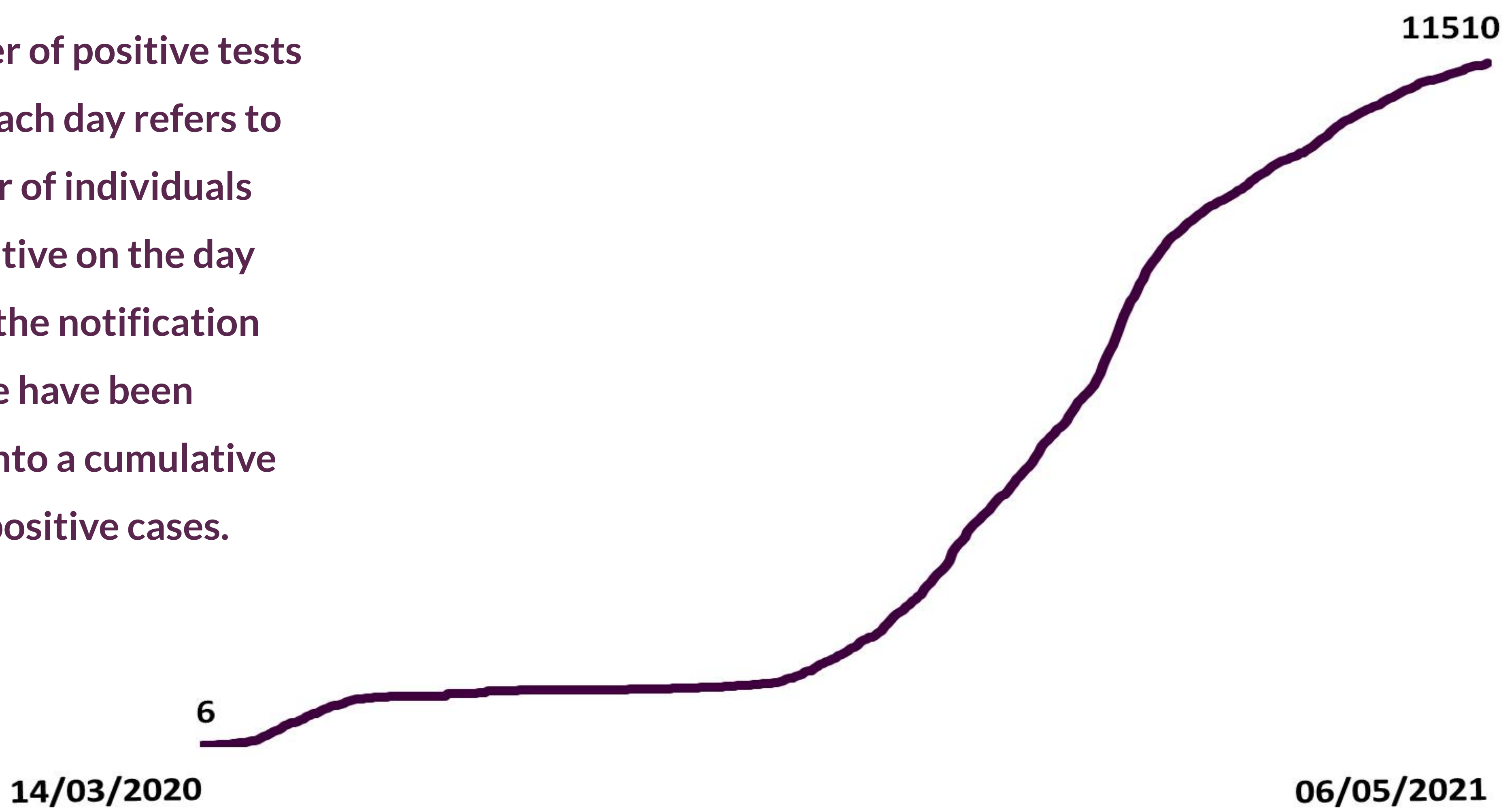
Cumulative confirmed COVID-19 cases, Fife Residents
